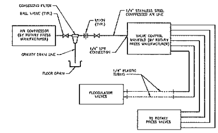
AIR COMPRESSOR SCHEMATIC NO SCALE
