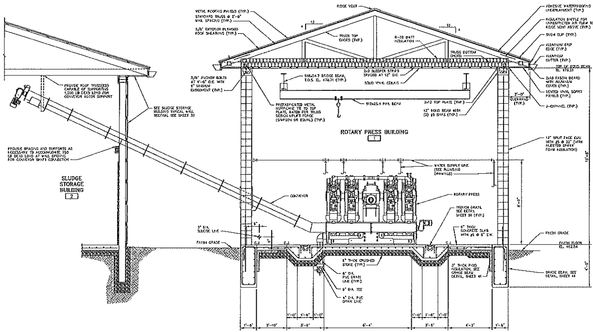
SECTION C-C - 40, 41, 42, 43, 44, 45 SCALE: 3/8" = 1'-0"
